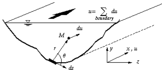
Fig. 1 The effect of a boundary element on the velocity of a point like M , in a river section
