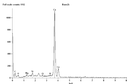
Fig. 10. EDAX of Ulva fasciata attached concrete surface in natural condition
