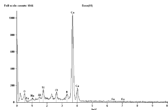
Fig. 11. EDAX of Ulva fasciata attached concrete surface in laboratory condition
