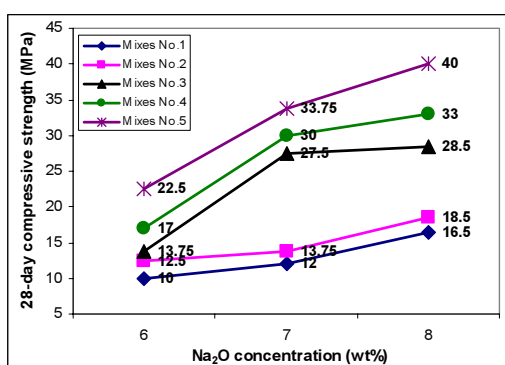
Fig. 4. Effect of \text{Na}_2\text{O} concentration on 28-day compressive strength
