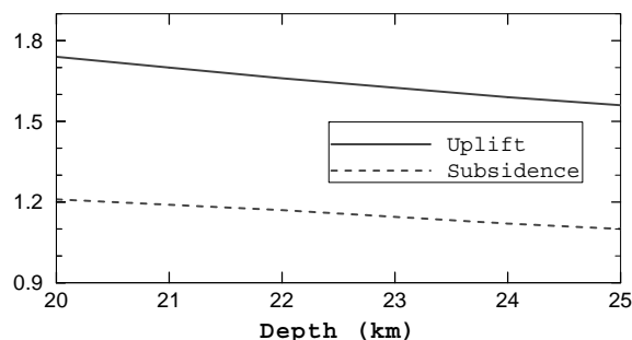
Fig.9 Maximum seafloor uplift and subsidence for different values of depth (Dip=7 deg, Slip Angle=90 deg, Displacement=6.15 m and Width=38 km)
