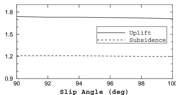
Fig.10 Maximum seafloor uplift and subsidence for different values of slip angle (Depth=20 km, and Dip=7 deg, Displacement=6.15 m and Width=38 km)
