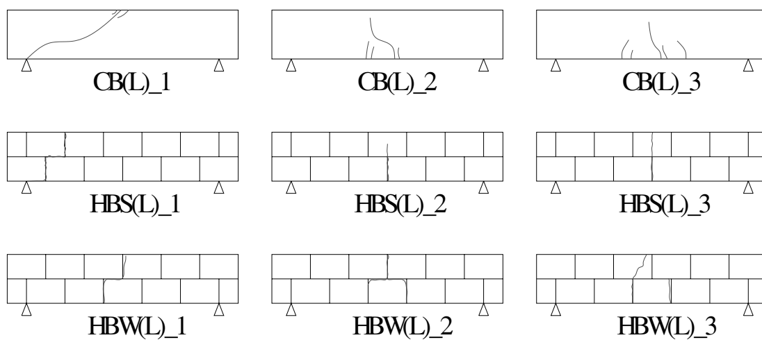
Fig. 2(b) Crack Patterns for Long Beams
