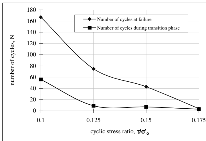
Figure 2. Number of cycles variation of transition and failure phases
