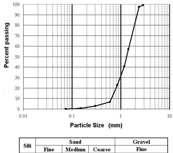
Fig. 3. Silica sand particle size distribution,
