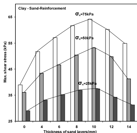
Fig. 10. Maximum shear stress layers versus thickness of sand layers for clay reinforced with thin layers of sand and reinforcement
