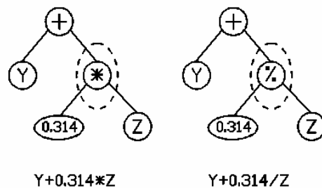
Fig. 3. Typical mutation operation in GP
