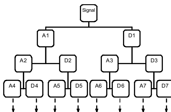
Fig. 2. Wavelet Packet decomposition tree
