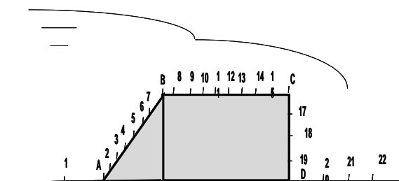
Fig. 2. Position of piezometer taps.
