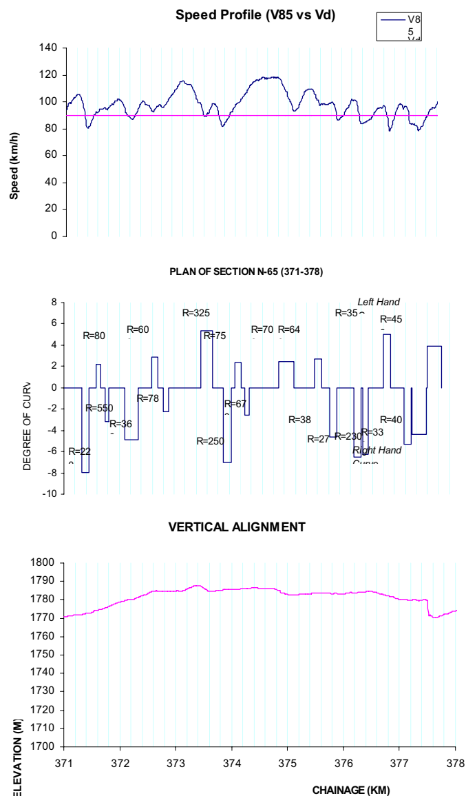
Fig. 2. Profiles of test section-I N-65 (371-378)
