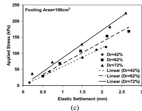
Fig. 6. Variation of applied stress versus elastic settlement for three sand relative densities (a) footing area of 25cm 2 , (b) footing area of 50cm 2 , and (c) footing area of 100cm 2 .
