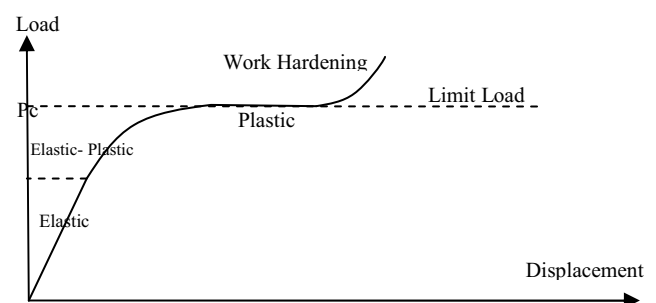
Fig. 1. Load-displacement curve
