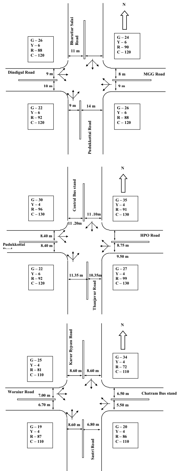
Fig. 1 Layouts of study intersection 1,2 and 3
