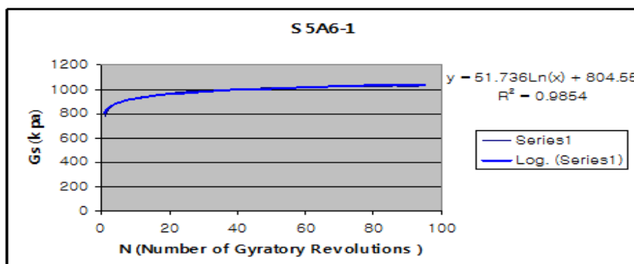
Fig. 5 Shear stress modeling versus gyration number (for one of the limestone specimens, gradation number 4, rock powder as the filler and 60-70 asphalt cement)
