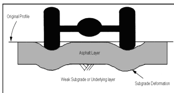
Fig. 1 Rutting due to bottom layers consolidation [5]
