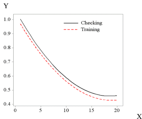
Fig. 9 Training process
